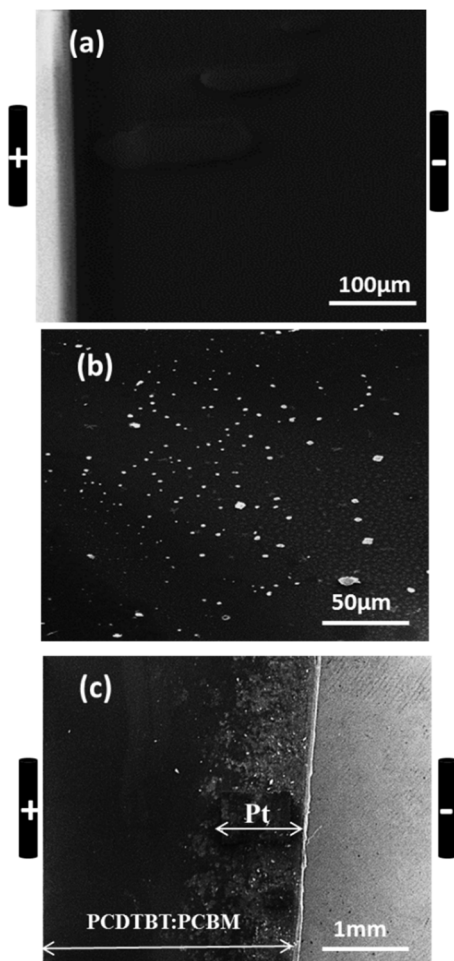
Fig. 1 SEM images of PCDTBT:PC 61 BM thin films after exposition (a) to only an external electric field, (b) only to light and (c) to light and an electric field of 2.8 \text{ kV m}^{-1} for 2 min in the presence of an aqueous solution of 1 \text{ mM H}_2\text{PtCl}_6 .
