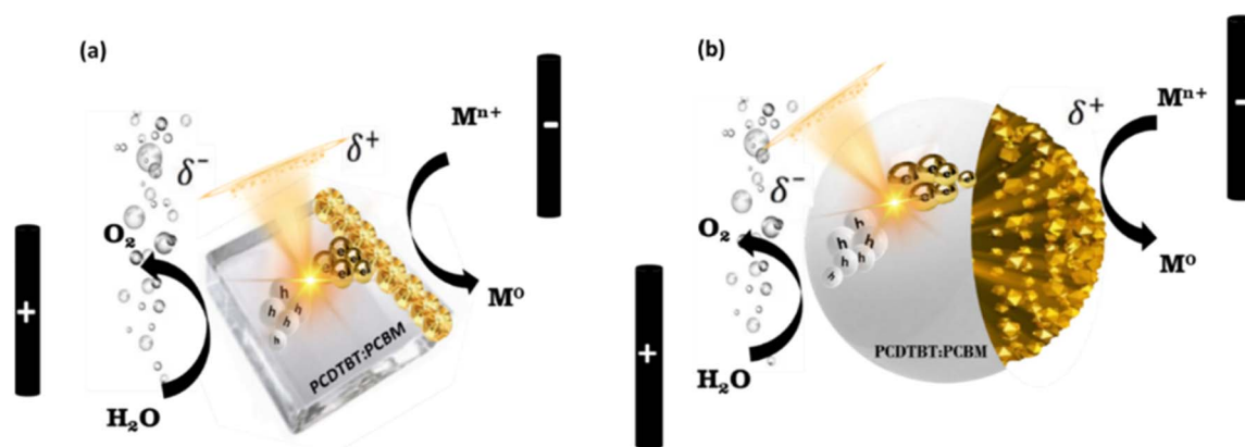
Scheme 1 Scheme of bipolar metal deposition on (a) a PCDTBT:PC 61 BM thin film and (b) a PCDTBT:PC 61 BM particle.
