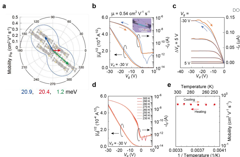
Fig. 3. Evaluation of MT-coronene as a semiconducting material. (a) Calculated \mu_{\text{hop}} and estimated mobility based on the hopping model. (b) Transfer and (c) output characteristics of SC-FET of MT-coronene measured in air. (d) Transfer characteristics measured at various temperatures in a vacuum. (e) Temperature dependence of carrier mobility.
