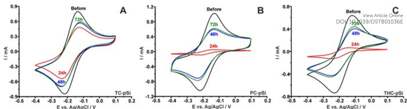
Figure 3. Cyclic voltammograms obtained using (A) TC-pSi, (B) PC-pSi, and (C) THC-pSi as working electrode, measured at different stages of biofilm growth, in the presence of 10 mM Ruhex. Electrolyte: 100 mM PBS. Scan rate: 0.1 V s -1 .
