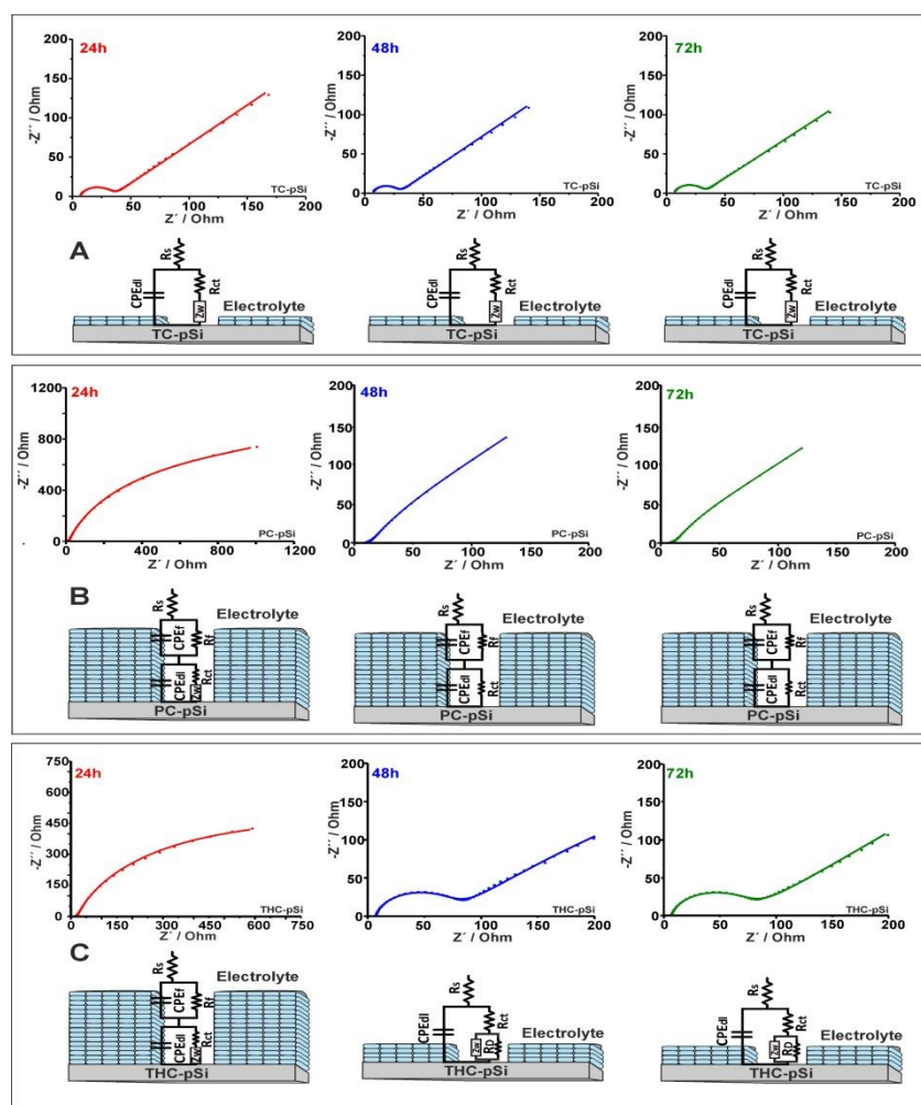
Figure 6. Nyquist plots obtained using (A) TC-pSi, (B) PC-pSi, and (C) THC-pSi as working electrode, measured at different stages of biofilm growth, in the presence of 10 mM Ruhex. Graphical illustrations of the biofilm growth state along with the respective equivalent circuits are included under each plot. Electrolyte: 100 mM PBS. DC potential: -0.2 V.
