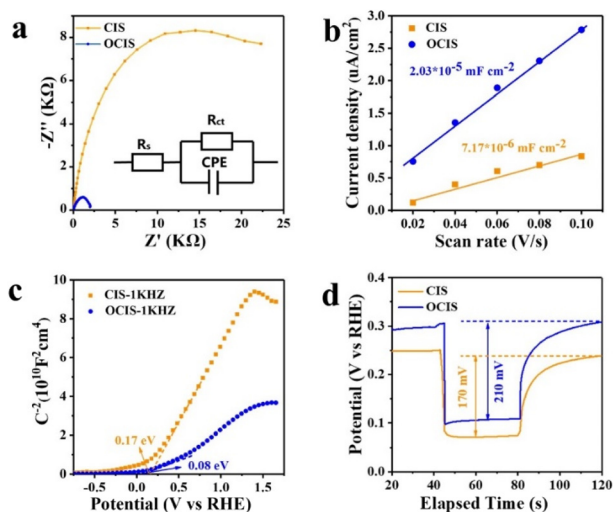
Fig. 5 (a) The EIS Nyquist plots for CIS and OCIS under illumination. (b) Current densities of CdS for CIS and OCIS. (c) M–S plots for CIS and OCIS in dark. (d) OCP measurements under dark and light conditions for CIS and OCIS.
