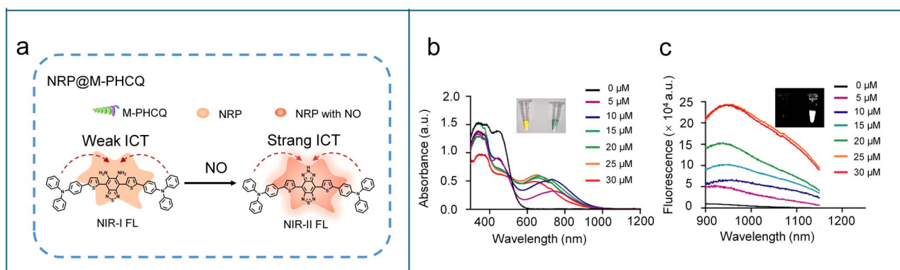
Fig. 4 (a) Reaction mechanism of NRP@M-PHCQ with NO. Absorbance (b) and fluorescence (c) of NRP@M-PHCQ after the addition of NO concentrations (5–30 μM). The insets show the photos of NRP@M-PHCQ before (left) and after (right) the addition of NO (30 μM). Reproduced from ref. 72 with permission from American Chemical Society, copyright 2023.
