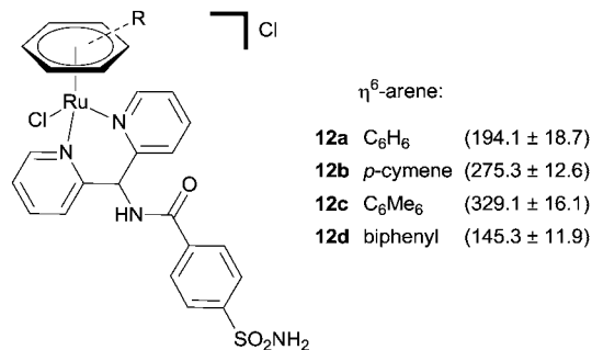
Fig. 7 A series of piano-stool Ru(II) arene CA inhibitors with inhibition constants (nM, K s ) in parenthesis (hCA II).
