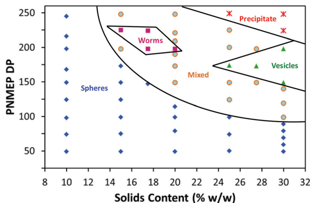
Fig. 5 Phase diagram for a series of PSMA 14 –PNMEP x diblock copolymers synthesised by RAFT dispersion polymerisation of NMEP in n -dodecane at various concentrations ranging between 10 and 30% w/w solids. Post-polymerisation analysis of each diblock copolymer dispersion by TEM determined the phase boundaries.
