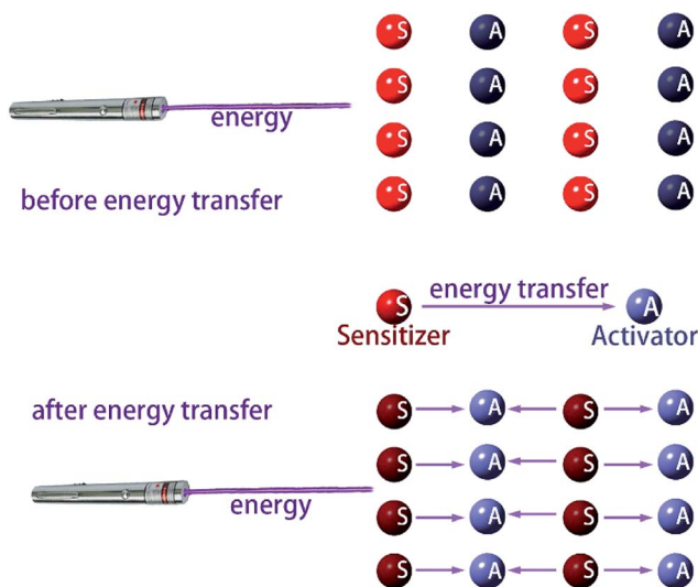
Fig. 13 Schematic diagram of the energy transfer, the dark and light colors indicate the level of energy.
