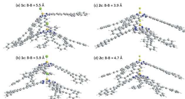
Fig. 10 Optimized structures of dimeric subnaphthalocyanines 1c and 2c . (a) 1c , B–B distance of 5.5 \text{\AA} , (b) 1c , B–B distance of 5.9 \text{\AA} , (c) 2c , B–B distance of 3.9 \text{\AA} , and (d) 2c , B–B distance of 4.7 \text{\AA} .
