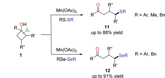
Scheme 16 The manganese-mediated ring-opening \text{C}(\text{sp}^3)\text{--S}/\text{C}(\text{sp}^3)\text{--Se} bond formation.
