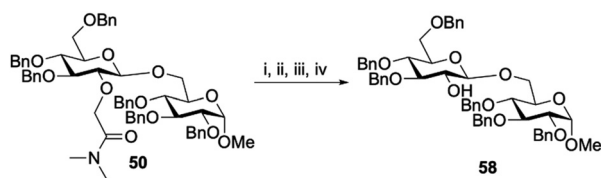
Scheme 1 Removal of the auxiliary. Reagents and conditions (i) \text{H}_2\text{O} (2.2 eq.), t\text{-BuOK} (5.9 eq.), THF, rt; (ii) DIPEA (1.2 eq.), DPPA (1.1 eq.), DMF, 0^\circ\text{C} – rt; (iii) t\text{-BuOH} , DMF, 100^\circ\text{C} ; (iv) \text{NaOH} , THF, EtOH, 60^\circ\text{C} .
