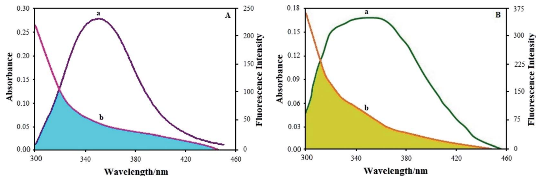
Fig. 11 (A) Overlap of the fluorescence spectrum of BSA ( T = 298\text{ K} ) and the UV absorption spectrum of the Ho(III) complex: (a) fluorescence spectrum of BSA; (b) UV absorption spectrum of the Ho(III) complex. (B) Overlap of the fluorescence spectrum of HSA ( T = 298\text{ K} ) and the UV absorption spectrum of the Ho(III) complex: (a) fluorescence spectrum of HSA; (b) UV absorption spectrum of the Ho(III) complex.
