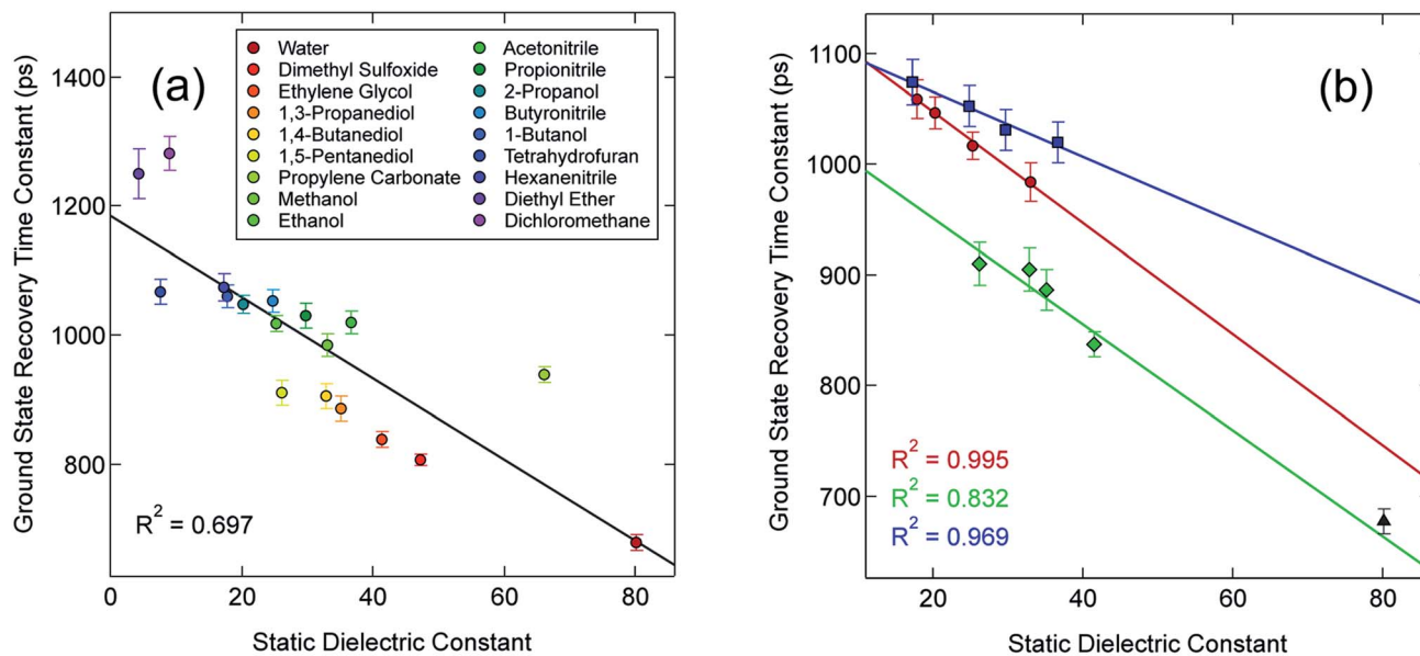
Fig. 2 (a) Time constants for ground state recovery of [\text{Fe}(\text{bpy})_3]^{2+} following ^1A_1 \rightarrow ^1\text{MLCT} excitation at 550 nm as a function of the static dielectric constant of the solvent. (b) A subset of the data from (a) grouped according to solvent type, specifically alcohols (red circles), diols (green diamonds), and nitriles (blue squares). The black triangle corresponds to data acquired in aqueous solution (a typical solvent choice in the literature for this complex), but is not included in any of the fits for reasons to be discussed later.
