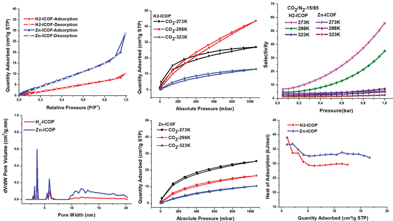
Fig. 4 (a) Kr adsorption/desorption isotherms of H2-ICOP and Zn-ICOP measured at 77 K, filled and empty symbols represent adsorption and desorption, respectively. (b) Pore size distribution of H2-ICOP and Zn-ICOP calculated from Kr isotherms calculated using NLDFT. \text{CO}_2 adsorption isotherms of H2-ICOP (c) and Zn-ICOP (d) collected up to 1 bar at 273, 298, and 323 K. (e) \text{CO}_2/\text{N}_2 (IAST method) selectivity of H2-ICOP and Zn-ICOP at 273 K, 298 K, and 323 K. (f) The isosteric heat of adsorption ( Q_{st} ) plots of \text{CO}_2 for H2-ICOP and Zn-ICOP .
