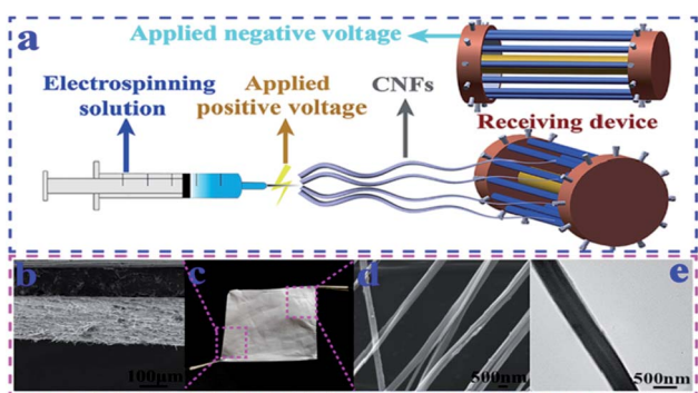
Fig. 1 (a) Improved electrospinning receiving device. (b) SEM image of the cross section of the cellulose nanofiber mat. (c) Photo of a piece of the cellulose nanofiber mat. (d) SEM image of CNFs. (e) TEM image of CNFs (reprinted with permission, 23 Elsevier publishing).
