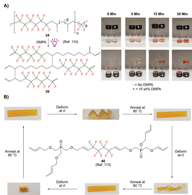
Fig. 8 Cross-linked iodo-ene polymers. (A). The use of 2,2-dimethoxy-1,2-diphenylacetophenone (DMPA) and 365 nm light to cross-link iodo-ene polymers into fluorinated gels (39). (B) Annealed cross-linked iodo-ene polymer 40 demonstrating enhanced shape memory and facile deformation. Reproduced from ref. 113 with permission from the American Chemical Society, Copyright 2019.
