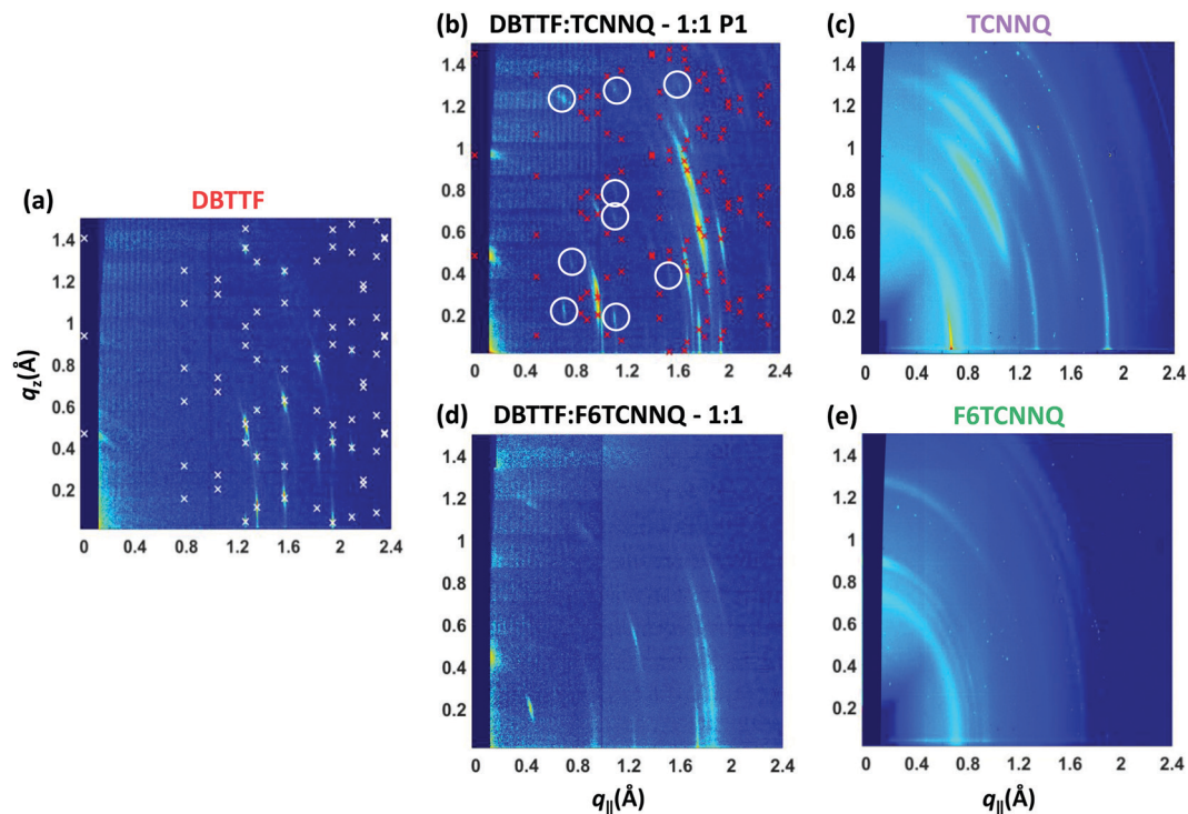
Fig. 6 X-ray scattering reciprocal space maps for single component D and A films of DBTTF (a), TCNNQ (c) and F6TCNNQ (e) as well as for co-deposited D:A films of DBTTF:TCNNQ (b) and DBTTF:F6TCNNQ (d). The measurements were performed on the same samples as the XRR measurements in Fig. 5. The presence of the respective polymorphs in these co-deposited DBTTF:TCNNQ films was determined by optical absorption measurements. The X-ray diffraction pattern related to the calculated crystal structure solution of the DBTTF thin film phase and of the mixed crystal polymorph P1 in co-deposited DBTTF:TCNNQ films are marked by crosses. The circles mark weak diffraction peaks probably related to the much less abundant P2 polymorph, whose features however are not visible either in XRR or optical absorption spectra. The unit cell parameters are given in Table 2. The ring at q_{\text{tot}} \approx 0.7 \text{ \AA}^{-1} for the single component acceptor films stems from the Kapton window of the sample holder.
