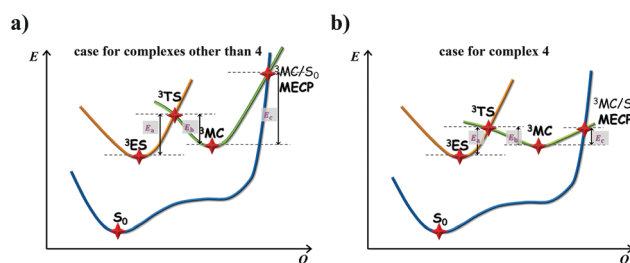
Fig. 5 Schematic representation of the competing excited-state deactivations of (a) complexes other than 4 that either ^3\text{TS} is high or MECP is unreachable; (b) complex 4 that both ^3\text{TS} and MECP are low in energy.
