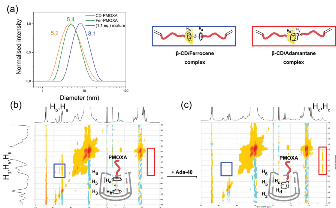
Fig. 3 (a) Size distribution of CD-PMOXA, Fer-PMOXA and their 1 : 1 molar mixture in at 25^\circ\text{C} ( c = 1\text{ g mL}^{-1} ). (b) 2D NOESY spectrum of 1 : 1 molar mixture of CD-PMOXA and Fer-PMOXA ( 5\text{ mmol L}^{-1} ) in \text{D}_2\text{O} at 30^\circ\text{C} and (c) 2D NOESY spectrum after the addition of Ada-40 (Adamantane-PMOXA).
