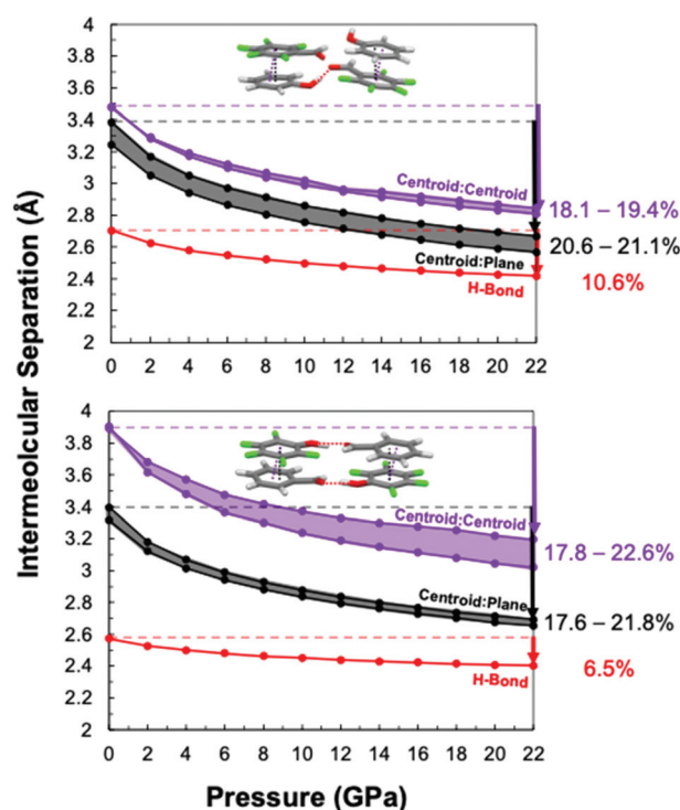
Fig. 2 Measured intermolecular interactions of simulated compressed co-crystals up to 22 GPa. Distances include centroid:centroid d_c (purple), centroid:plane d_p (black), and intra-stack O\cdots O hydrogen bonding (red) of each co-crystal ArOH:ArFCHO (top) and ArCHO:ArFOH (bottom).
