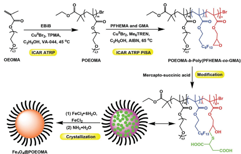
Fig. 6 Preparation scheme of \text{Fe}_3\text{O}_4 nanoparticles within the block copolymer nano-objects. Reproduced with permission from ref. 133. Copyright © 2019 WILEY-VCH Verlag GmbH & Co. KGaA, Weinheim.
