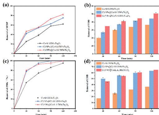
Fig. 5 Removal of organic phosphines by three catalysts: removal of HEDP (a) and its COD (b), and removal of PMG (c) and its COD (d).
