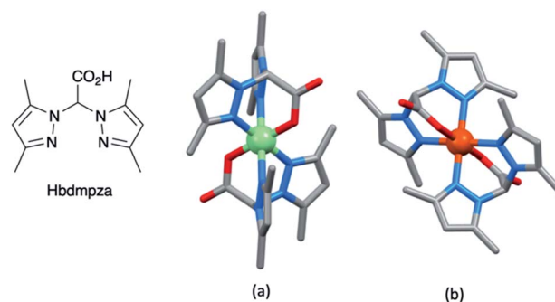
Fig. 5 The conjugate acid of the heteroscorpionate ligand [bdmpza] 2- and the structures of (a) the manganese(III) complex [Mn(bdmpza) 2 ] + (CSD refcode ITEQOP) and (b) the iron(III) complex [Fe(bdmpza) 2 ] + (refcode ITEQEF) both in the [BF 4 ] - salts.
