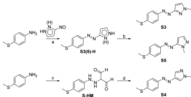
Scheme 1 Synthesis routes of 4-methylthioarylazopyrazoles. Reagent and conditions. (a) AcOH, room temperature, 58%. (b) CH 3 I, Cs 2 CO 3 , DMF, room temperature, 89%. (c) AcOH, concentrated HCl, aqueous NaNO 2 , 0–5 °C, aqueous KOAc, malonaldehyde sodium salt (MDA-Na), 0–5 °C, 54%. (d) Methylhydrazine sulfate, KOAc, EtOH, reflux, 74%.
