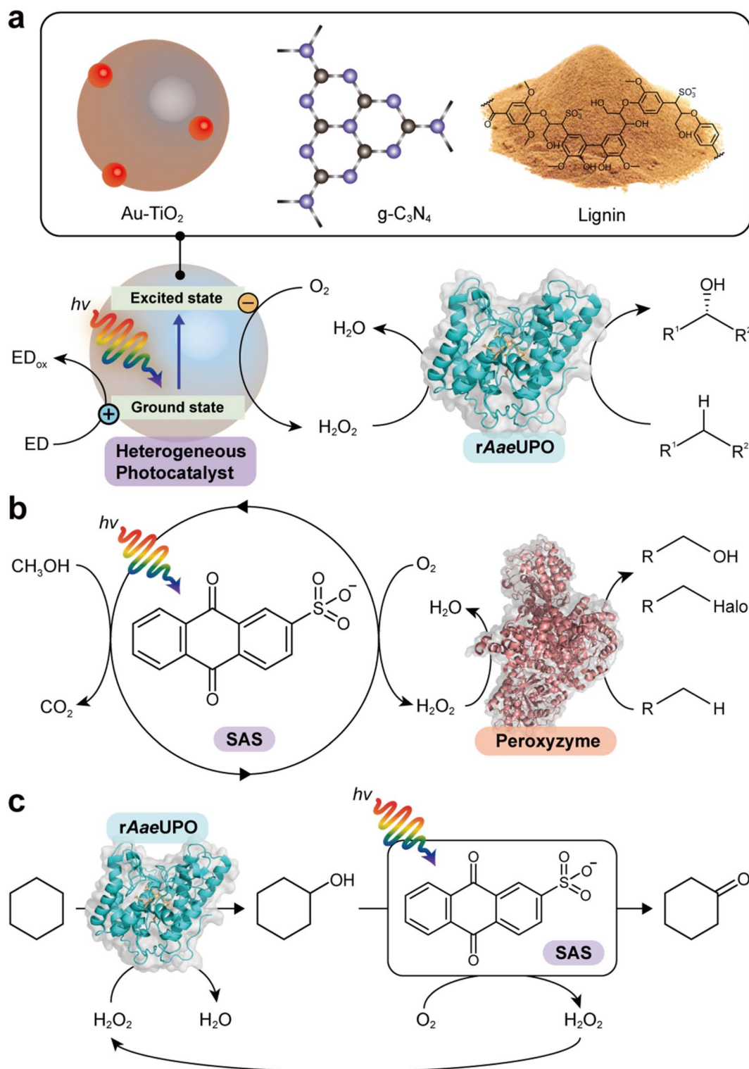
Fig. 6 Photocatalytic formation of \text{H}_2\text{O}_2 and selective oxidation reactions catalyzed by rAaeUPO and peroxyzyme. Representative photocatalysts include \text{Au-TiO}_2 , 90 \text{g-C}_3\text{N}_4 , 93 lignin 99 (a), and anthraquinone (SAS) 97,106 (b). (c) Photocatalytic oxidation of cyclohexane to cyclohexanone. The SAS-catalyzed aerobic overoxidation of cyclohexanol to cyclohexanone produces \text{H}_2\text{O}_2 as a byproduct, which itself is used to support the rAaeUPO-catalyzed hydroxylation of cyclohexane. 97
