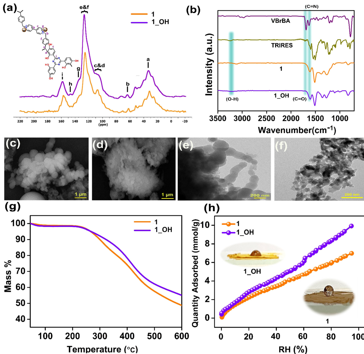
Fig. 1 (a) 13 C-CPMAS spectra of 1 and 1_OH ; (b) IR spectra of TRIRES, VBrBA, 1 , and 1_OH ; (c and d) FESEM images of 1 and 1_OH ; (e and f) HRTEM images of 1 and 1_OH ; (g) thermogravimetric analysis of 1 and 1_OH under N 2 atmosphere at a ramp rate of 5 °C min -1 ; and (h) water adsorption isotherms of 1 and 1_OH with insets presenting photographs from the contact angle measurements.
