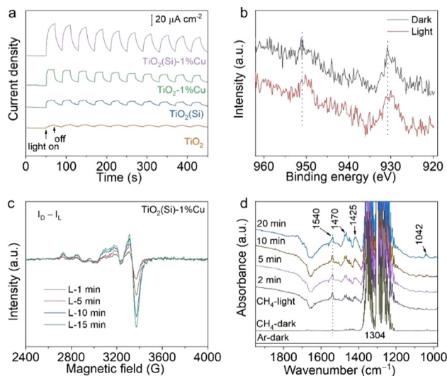
Fig. 4 (a) Transient photocurrent response of the prepared \text{TiO}_2 nanosheets. (b) The light-irradiated Cu 2p XPS spectra for \text{TiO}_2(\text{Si})-1\% \text{Cu} . (c) The EPR difference spectra between light irradiated spectra and pristine spectrum for \text{TiO}_2(\text{Si})-1\% \text{Cu} . (d) In situ DRIFTS spectra for photocatalytic methane conversion over \text{TiO}_2(\text{Si})-1\% \text{Cu} under light irradiation.
