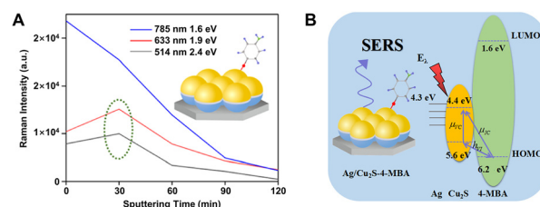
Fig. 10 (A) Intensity of Raman peak at 1586 \text{ cm}^{-1} of 4-MBA on Ag/Cu 2 S hemispherical dual-shell with various excitation wavelengths and sputtering times and (B) the corresponding coupling scheme in this Ag/Cu 2 S/4-MBA system. Reproduced from ref. 195 with permission from American Chemical Society, copyright 2018.
