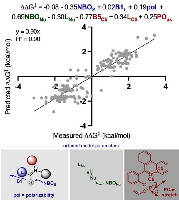
Fig. 4 The published statistical model describing the chiral phosphate catalysed nucleophilic addition to iminium intermediates. ' NBO_S ' and ' NBO_{Nu} ' are the natural bond orbital parameters corresponding to the first atom of the iminium small group (usually a hydrogen) and the nucleophilic site (either a carbon, hydrogen, oxygen, or nitrogen), ' B1_L ' is the minimum width (Sterimol B1) of the largest iminium substituent, ' pol ' is the calculated polarizability of the iminium, ' L_{Nu} ' is the nucleophile length (Sterimol L), B5_{C5} is the maximum width (Sterimol B5) of the catalyst 5-substituent, L_{C6} is the length of the catalyst 6-substituent, and finally ' PO_{as} ' is the asymmetric P–O stretching frequency.
