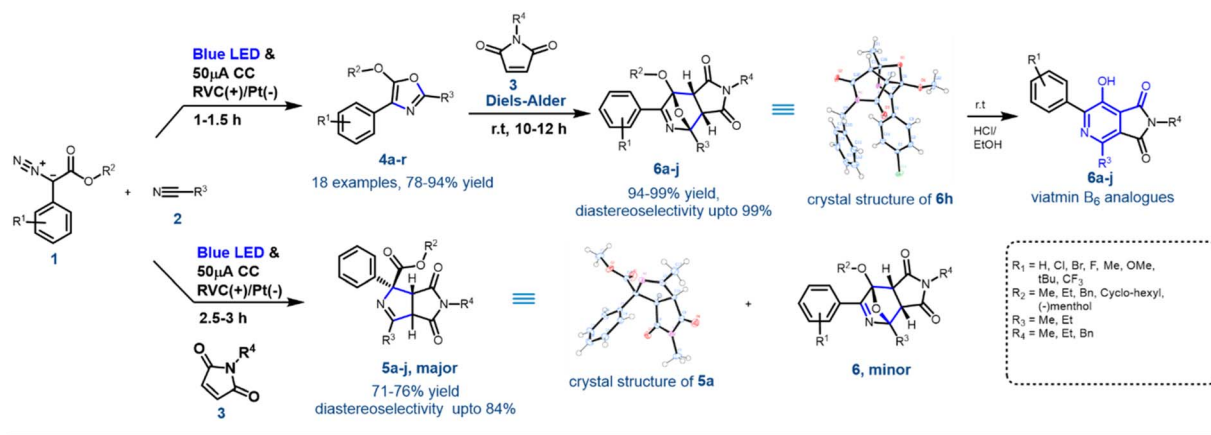
Scheme 1 General scheme of the EPC reaction and further synthetic application.
