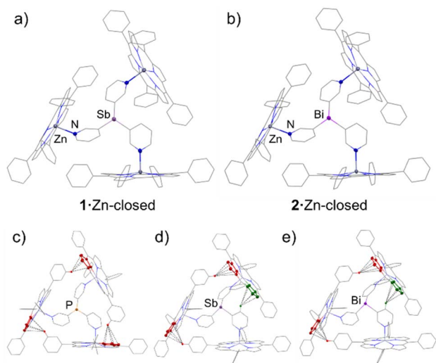
Fig. 4 X-ray structures of the complexes 1 ·Zn-closed (a) and 2 ·Zn-closed (b). In both structures, the ligand coordinates three porphyrins leading to the formation of capsule-type structures. Solvent molecules and H-atoms are omitted for clarity. Selected bond lengths (Å) and angles (°): 1 ·Zn, Sb–C py range 2.146(5)–2.158(5); N py –Zn range 2.149(4)–2.194(4); C py –Sb–C py range 95.4(2)–96.0(2). 2 ·Zn, Bi–C py range 2.235(6)–2.261(5); N py –Zn range 2.149(5)–2.184(5); C py –Bi–C py range 93.0(2)–94.2(2). Colour key: C (grey), Zn (dark grey), N (blue), P (orange), Sb (light purple), Bi (purple). X-ray structures of [\text{P}(3\text{-py})_3] \cdot (\text{ZnTPP})_3 (c), 1 ·Zn (d) and 2 ·Zn (e) showing the capsules with close intramolecular CH– \pi interactions between ZnTPP building blocks highlighted in red and interactions between C–H pyridyl and ZnTPP highlighted in green. CH– \pi interaction lengths (Å): [\text{P}(3\text{-py})_3] \cdot (\text{ZnTPP})_3 2.725, 2.893 and 2.960; 34 1 ·Zn 2.971, 3.051 and 2.978 (CH py – \pi ); 2 ·Zn 2.991, 3.025 and 2.978 (CH py – \pi ).
