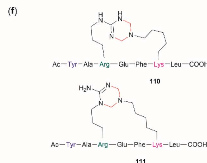
Fig. 22 (a) Chemoselective Tyr protein functionalization with formaldehyde and aromatic amines as reported by Joshi et al. 105 (b) Lys-Tyr stapling protocol described by Li et al. 106 (c) Effect of the number of residues between Lys and Tyr in the efficacy of the stapling reaction after 1 h. (d) Peptide systems selected to exemplify the closest Lys-Tyr pair reactivity. (e) Products of the stapling between the N-terminal amino group and Tyr. (f) Formaldehyde mediated stapling reaction between Arg and Lys residues.
