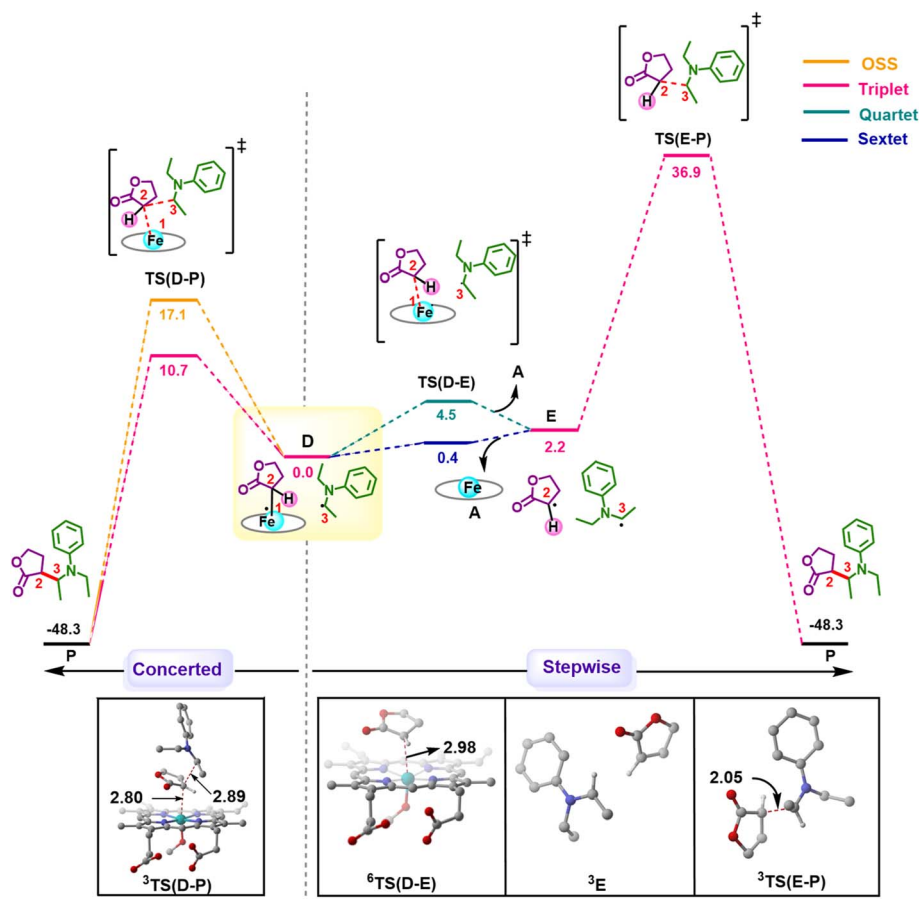
Fig. 2 Gibbs free energy profile (kcal mol -1 ) for comparison of concerted and stepwise pathways for C–H insertion at different spin states of Fe. Distances are in Å. The H atoms are omitted for clarity.
