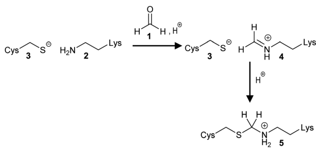
Scheme 1 Formation of the methylene bridge 5 using methanal 1 . The Mannich reaction proceeds via formation of an imine intermediate 4 .
