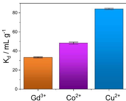
Fig. 5 Distribution coefficient ( K_d ) values of the MONO-DTPA samples used in the capture of the \text{Gd}^{3+} , \text{Cu}^{2+} and \text{Co}^{2+} ions from 10 mM aqueous solutions (the bars represent the mean value and the error bars indicate the standard deviation; n = 3 ).
