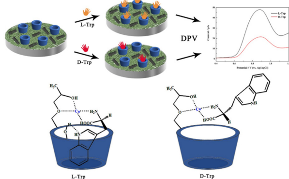
Fig. 7 Schematic representation of the electrochemical chiral recognition of tryptophan isomers (reprinted from ref. 81 with permission from Elsevier).
