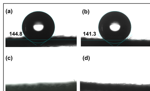
Fig. 2 Hydrophilicity test of CC after different pretreatment processes: (a) original CC; (b) treated with KOH; (c) treated with \text{HNO}_3/\text{H}_2\text{SO}_4/\text{KMnO}_4 mixture; (d) treated with \text{H}_2\text{O}_2 .
