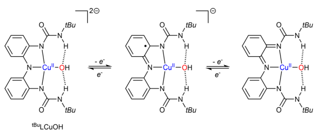
Scheme 9 Characterized oxidation states reached via reduction/oxidation of tBu_2CuOH . Adapted from ref. 73.
