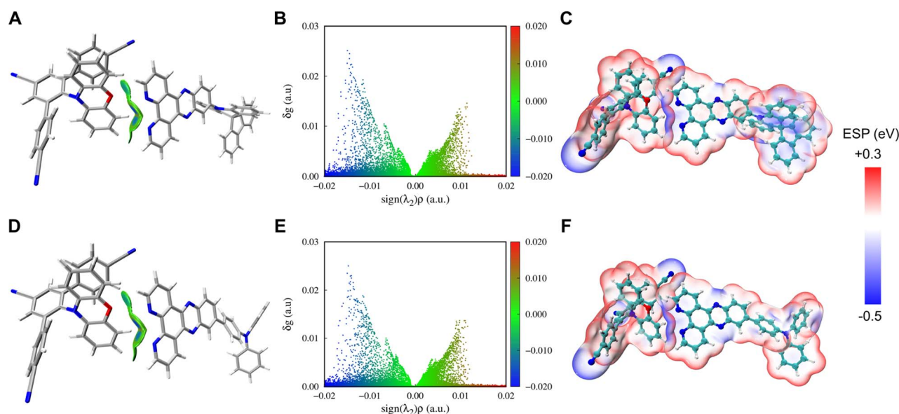
Fig. 3 Isosurface maps of intermolecular interaction based on optimized geometry (isovalence = 0.003 a.u., color range: \pm 0.02 a.u.), corresponding scatter plots and ESP maps of mPTBC : SAF-2NP (A–C) and mPTBC : TPA-2NP (D–F).
