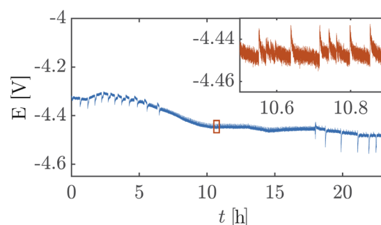
Fig. 5 Variation of cell voltage with time recorded during a chrono-potentiometry experiment performed with a platinum-coated PSi-ZGE with a pore size of 4.1 \mu\text{m} and porosity of 0.61% at a constant current of 100 mA cm -2 shows that PSi-ZGE does not materially degrade over the 24 hours. The fluctuations in potential due to bubble evolution are made clearer in the inset.
