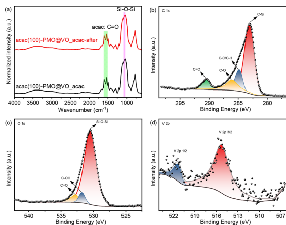
Fig. 7 (a) DRIFT spectra of acac(100)-PMO@VO 2 before and after Mannich-type reaction; (b) deconvoluted XPS C 1s spectra, (c) O 1s spectra and (d) vanadium in the V 2p region of the recycled acac(100)-PMO@VO 2 .
