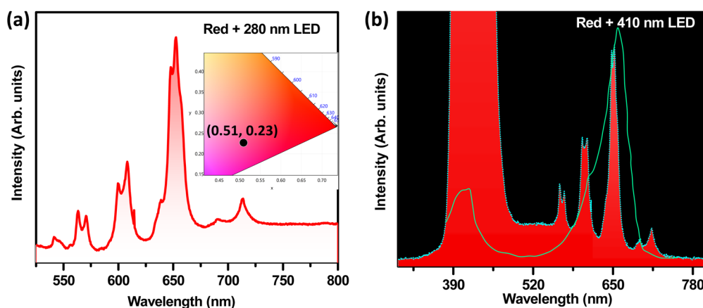
Fig. 10 (a) The electroluminescence spectra for the \text{Sc}_2\text{Mo}_3\text{O}_{12}:\text{Sm}^{3+} sample excited with 280 nm LED. The inset shows the chromaticity diagram for the same sample showing the CIE coordinates. (b) The electroluminescence spectra for the \text{Sc}_2\text{Mo}_3\text{O}_{12}:\text{Sm}^{3+} sample excited with 410 nm LED, along with the absorption spectra of the plant pigment phytochrome P_R .
