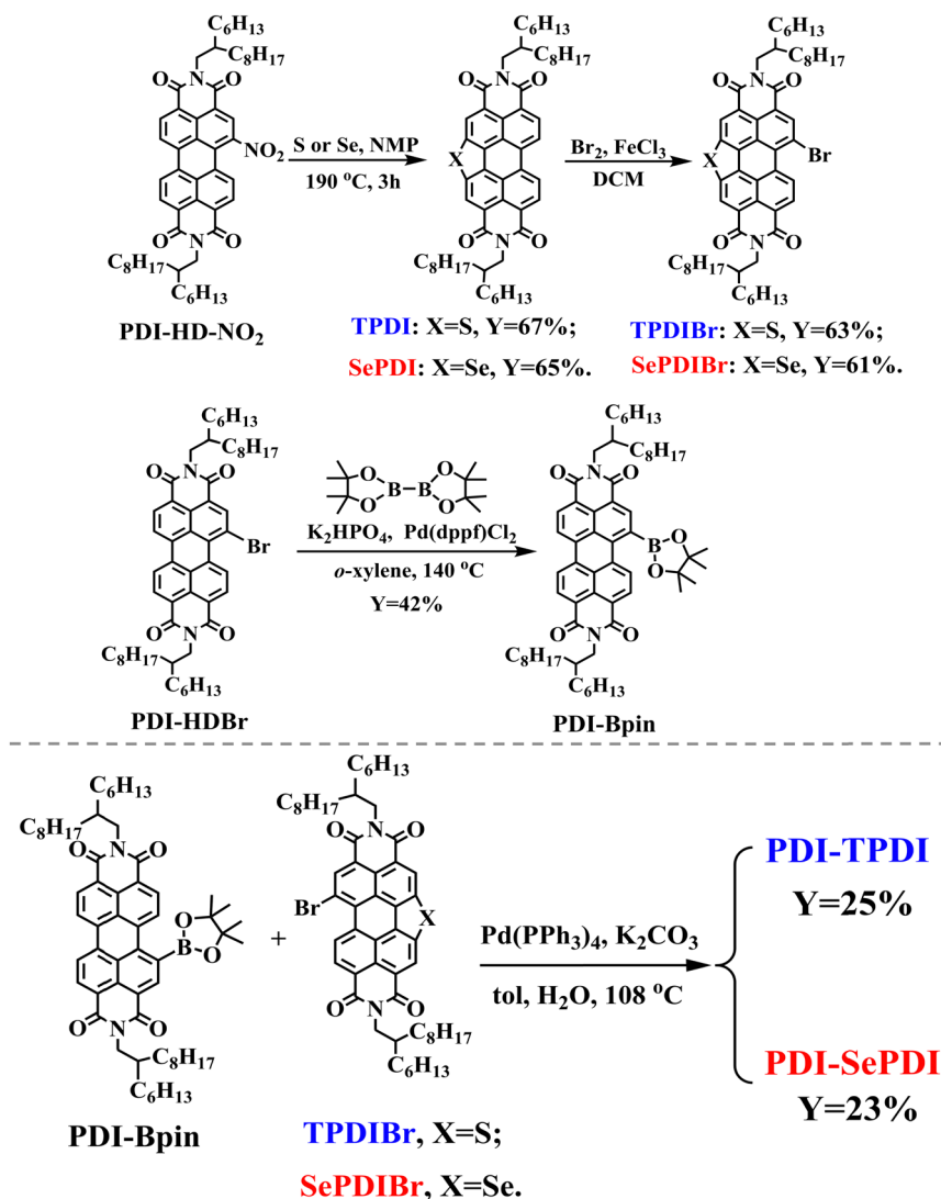
Scheme 1 Synthesis of monobromides TPDI Br and SePDl Br, monoboric ester PDI -Bpin and asymmetric PDI dimeric acceptors PDI -TPDI and PDI -SePDl.
