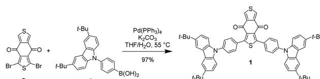
Scheme 1 Synthesis of compound 1 .
