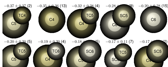
Fig. 8 Top ten most influential molecular features contributing to lipid bilayer phase separation, identified via LASSO regression of the optimized CG molecules with \Delta\Delta G < 0 . Features were limited to single beads and bead pairs. Each panel displays a feature's structure along with its corresponding regression coefficient, bootstrapped uncertainty, and frequency of occurrence within the dataset (number in parentheses). Features only involve hydrophobic C4, C5, and C6 beads and pairs of differing bead sizes.
