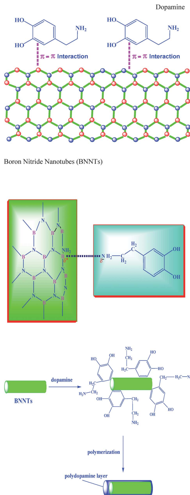
Scheme 1 Schematic illustration of dopamine functionalization of BNNTs.
