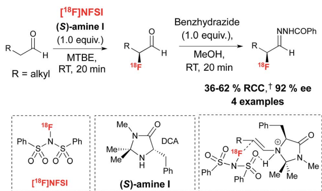
Scheme 5 Chiral imidazolidinone ( S )-I for the enantioselective ^{18}\text{F} -fluorination of aldehydes with [ ^{18}\text{F} ]NFSI. †RCC determined by radio-HPLC relative to [ ^{18}\text{F} ]NFSI. DCA = dichloroacetic acid. For [ ^{18}\text{F} ]NFSI, SA = 0.05 Ci \mu\text{mol}^{-1} , ( n = 3).
