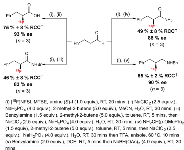
Scheme 6 Radiosynthesis of enantioenriched ^{18}\text{F} -labeled carboxylic acid, amides and amine. †RCC determined by radio-HPLC relative to [ ^{18}\text{F} ]NFSI.
