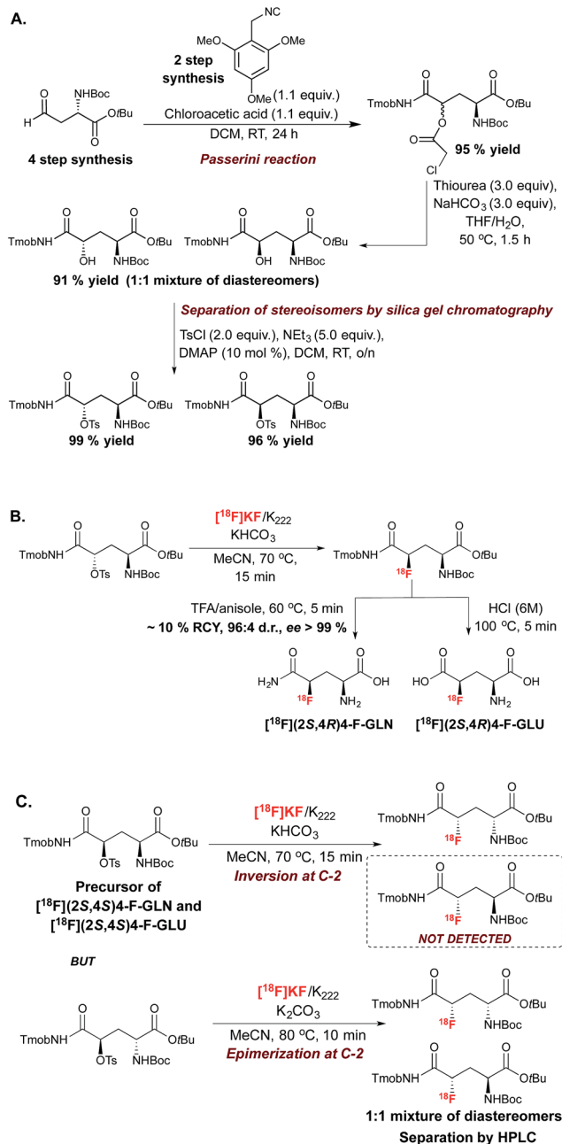
Scheme 2 (A.) Synthesis of the substrates for the radiosynthesis of [^{18}\text{F}]4\text{-F-GLU} and [^{18}\text{F}]4\text{-F-GLN} . (B.) Radiosynthesis of [^{18}\text{F}](2\text{S},4\text{R})4\text{-F-GLU} and [^{18}\text{F}](2\text{S},4\text{R})4\text{-F-GLN} . (C.) Radiosynthesis of [^{18}\text{F}](2\text{S},4\text{S})4\text{-F-GLU} and [^{18}\text{F}](2\text{S},4\text{S})4\text{-F-GLN} precursors. Tmob = 2,4,6-trimethoxybenzyl.
