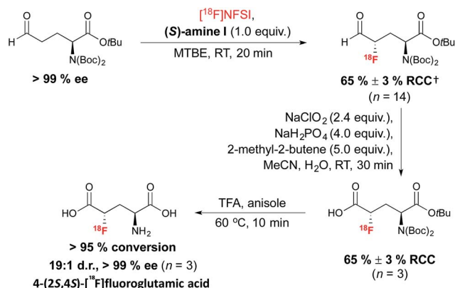
Scheme 7 Organomediated radiosynthesis of [ ^{18}\text{F} ](2S,4S)-4-F-GLU. †RCC determined by radio-HPLC relative to [ ^{18}\text{F} ]NFSI.
