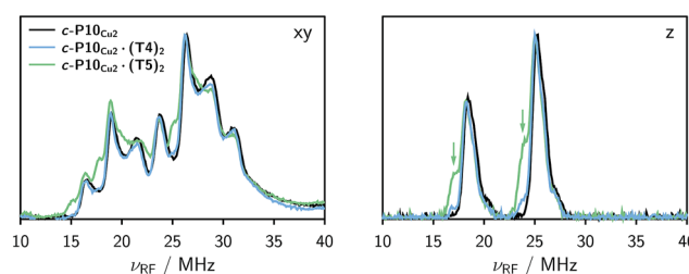
Fig. 4 Comparison of the 14 N Davies ENDOR spectra of all three samples recorded at field positions corresponding to the xy (left) and z (right) orientations in frozen toluene- d 8 at 15 K. The green arrows indicate the additional nitrogen hyperfine coupling observed for c-P10 Cu2 ·( T5 ) 2 .
