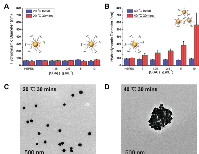
Fig. 3 Dynamic light scattering (DLS) analysis of thermally gated lectin binding. pHEA 15 -Gal:pNIPAM 50 ratio 9:1 @AuNP 60 . (A) Hydrodynamic diameter at 20\text{ }^{\circ}\text{C} initially, and after 30 minutes incubation with SBA; (B) hydrodynamic diameter at 40\text{ }^{\circ}\text{C} , initially and after 30 minutes incubation with SBA. All results are mean from a minimum of 3 independent repeats. TEM images of these particles after addition of SBA ( 10\text{ }\mu\text{g mL}^{-1} ): (C) at 20\text{ }^{\circ}\text{C} for 30 min; (D) at 40\text{ }^{\circ}\text{C} following 30 minutes incubation.
