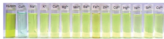
Fig. 2 Visual color change from yellow to sky blue on addition of \text{Cu}^{2+} ion in the aqueous solution of \text{H}_5\text{dpm} among different cations.
